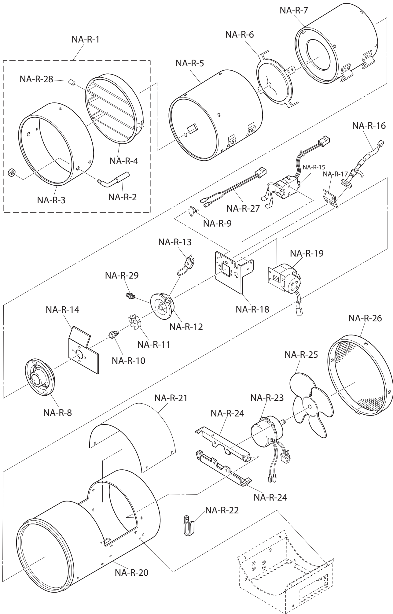
HG-125NA Main Section
