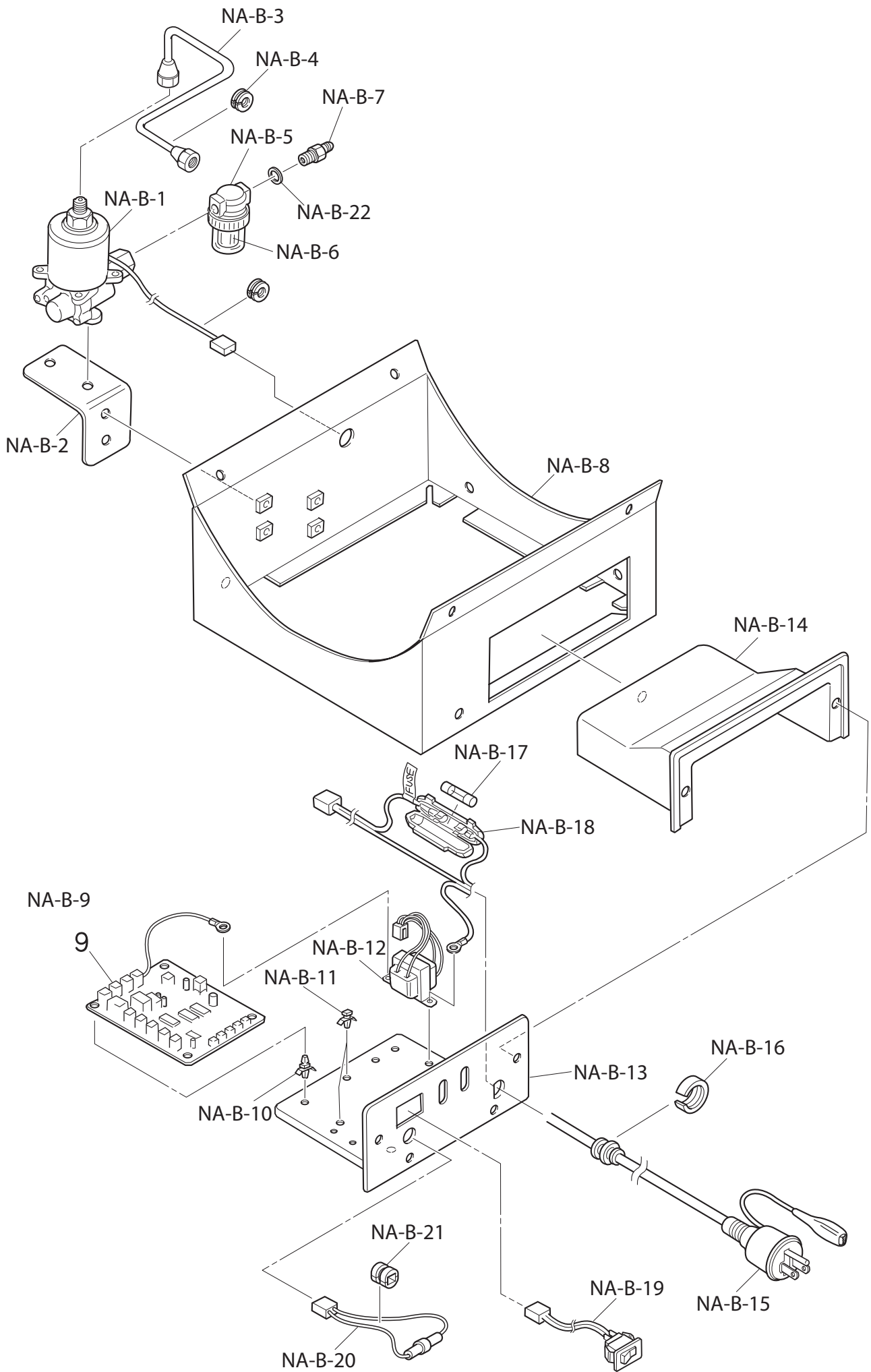
HG-125NA Control Section
